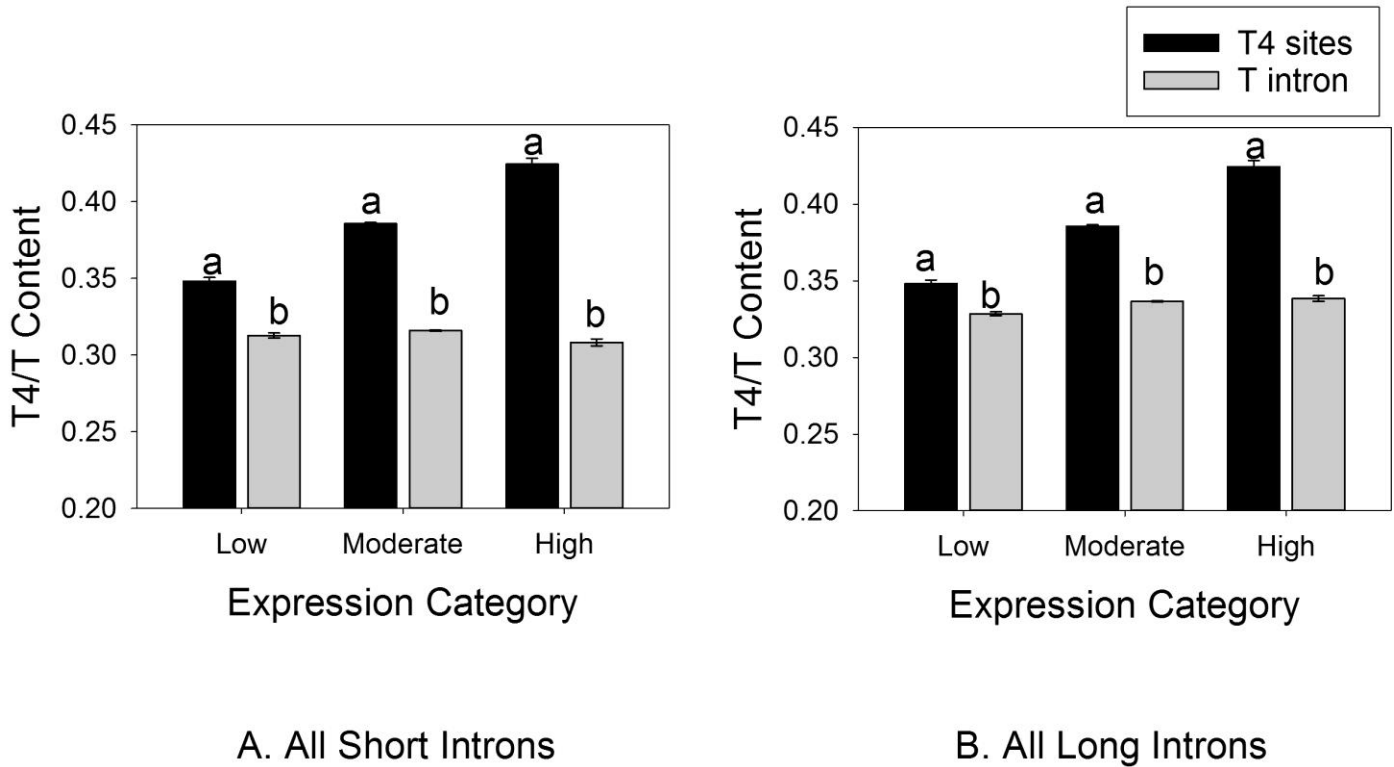
Figure S2. The T4 content of CDS and the T content of the associated introns per expression category. A) All short introns (unconcatenated) per expression class. B) All long introns per expression class. The 50bp at each end of long introns were removed prior to analysis. Different letters within an expression class indicate a statistically significant difference using MWU-tests ( P < 0.001 ).
